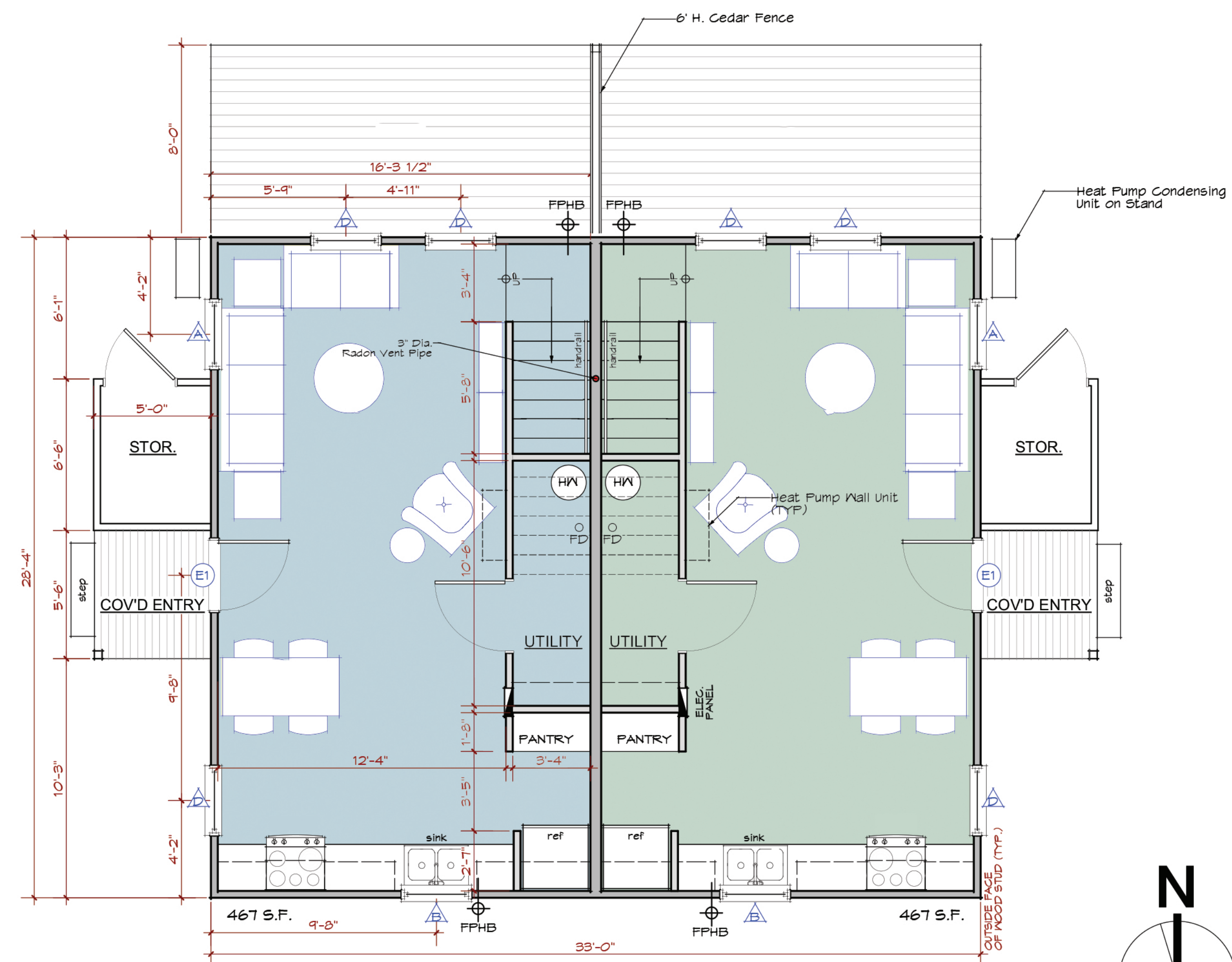
1 FIRST FLOOR PLAN A1.1 1/4" = 1'-0"
